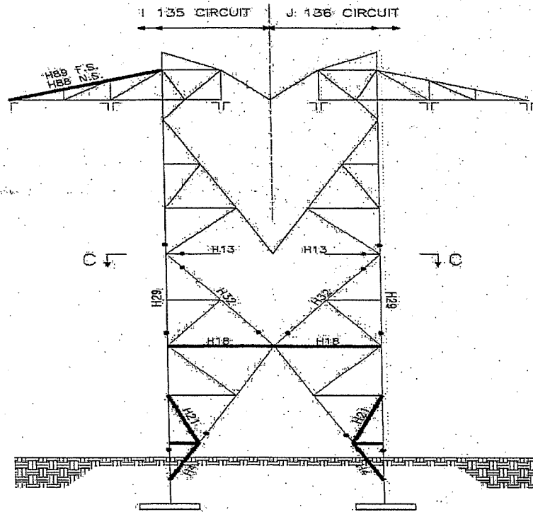
Figure 1: Lattice Tower
